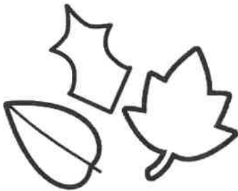
Leaves
